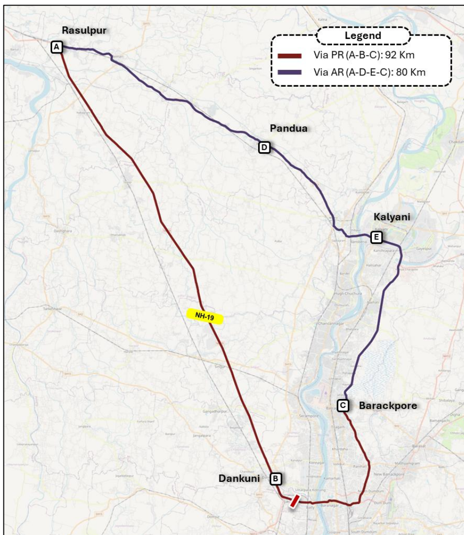
Figure 6-5: Alignment of PR and AR
