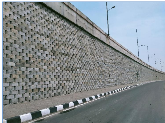
RE Blocks at Km 23+550 RHS
