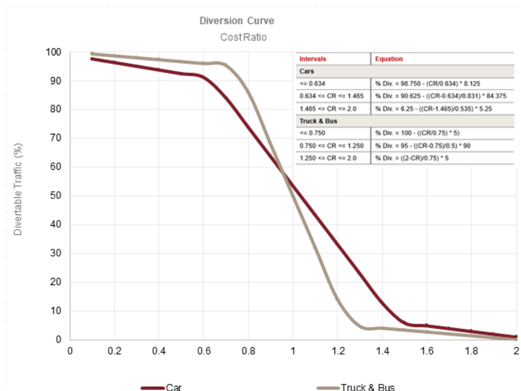
Figure 6-1: Diversion curve as per IRC:108-2015
