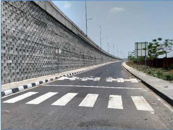
Service road at km 50.100 LHS
